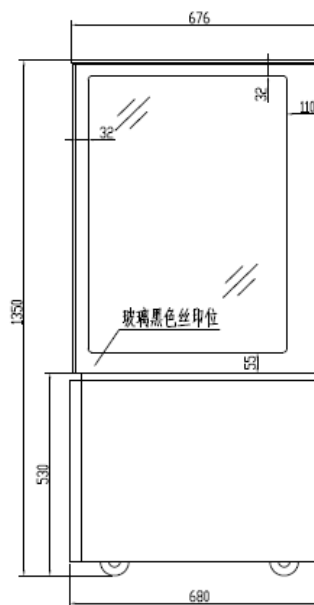
SIDE VIEW 左侧视图
