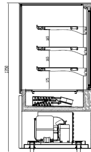
SECTION VIEW 左侧视图
