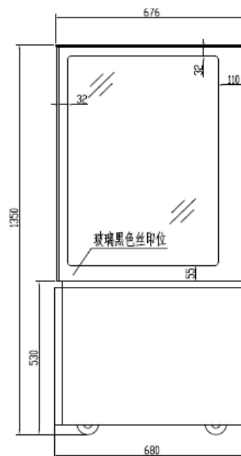
SIDE VIEW 左侧视图
