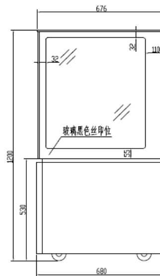
SIDE VIEW 左侧视图
