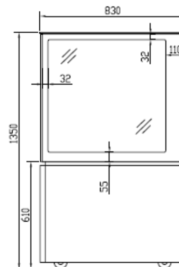
SIDE VIEW 左侧视图
