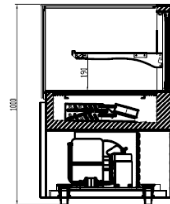
SECTION VIEW 左剖视图
