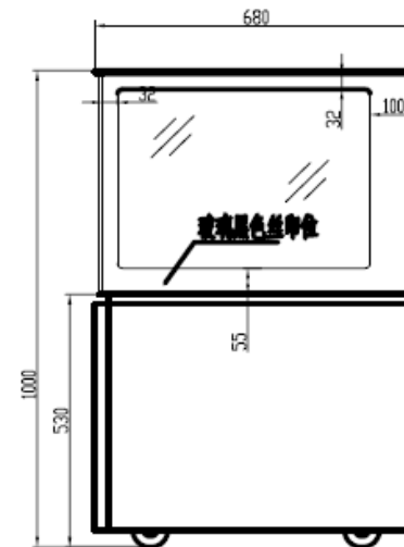
SIDE VIEW 左侧视图
