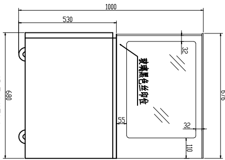
SIDE VIEW 左侧视图
