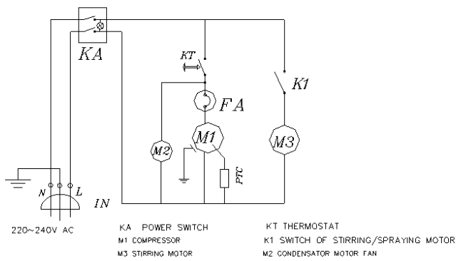
Electric Wiring Diagram
