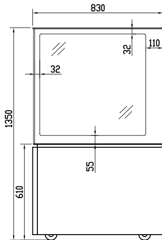
SIDE VIEW 左侧视图
